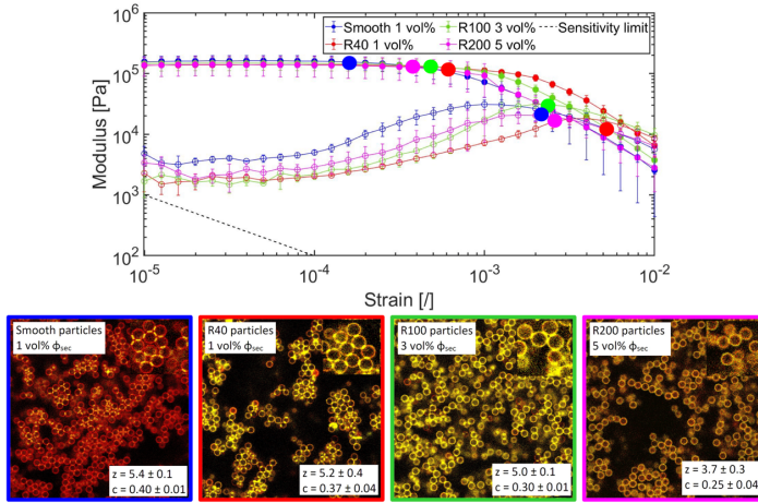
Figure 3: Influence of particle roughness for samples with secondary fluid volume adjusted to match the storage moduli. Increasing roughness increases the yield strain with very little effect on the flow point. The structure becomes less dense (decreasing both the coordination number and clustering coefficient) as the roughness increases.
