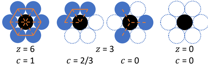
Figure 1: Difference between the coordination number z , the number of bonds per particle (dashed lines), and the clustering coefficient c . The clustering coefficient is defined as c = \frac{2e}{z(z-1)} , where the number of bonds between neighbors (solid lines) is e .
